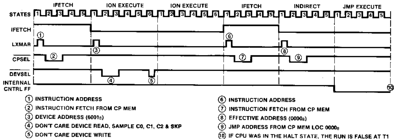
Figure 16: "ION; JMP I 0000" In Control Panel Routine
