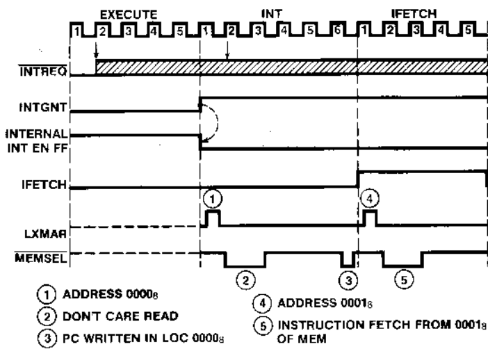
Figure 11: Device Interrupt Grant Timing
