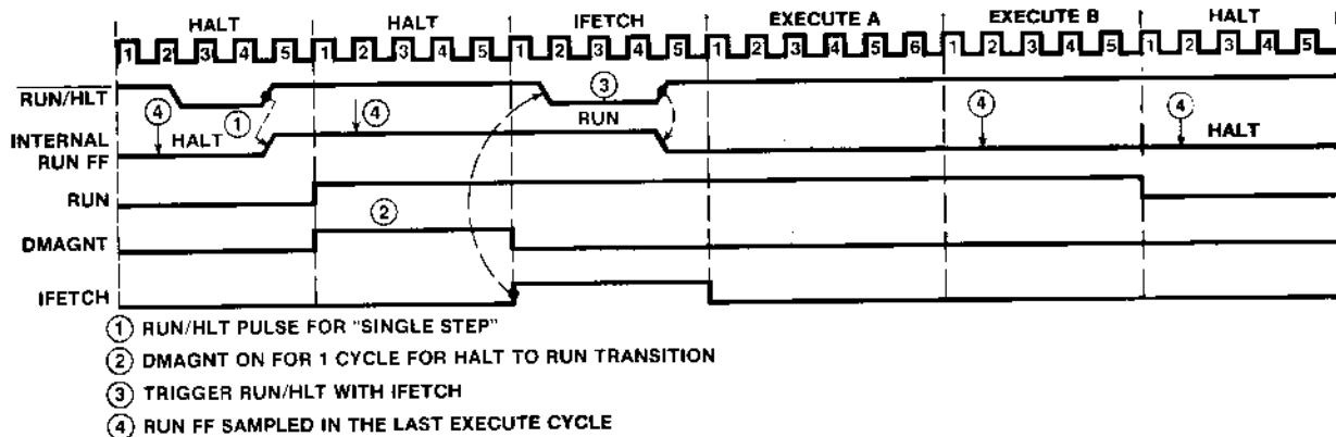
Figure 21: "Single Step" With Run/Halt
